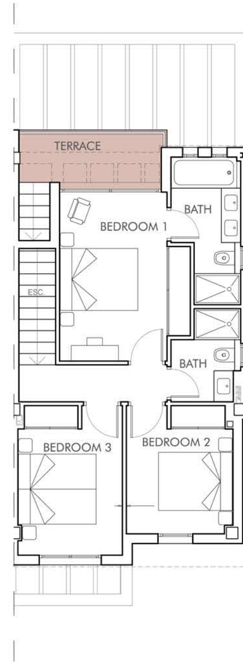
FIRST FLOOR
